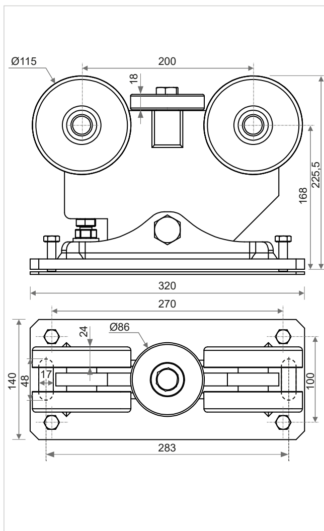
Chariot Rollco® LWS 125/L
