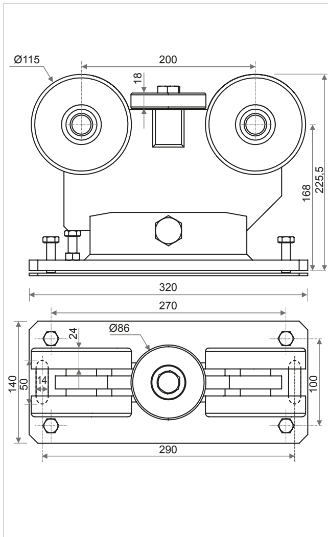
Rollenbock Rollco® LWS 125/S
